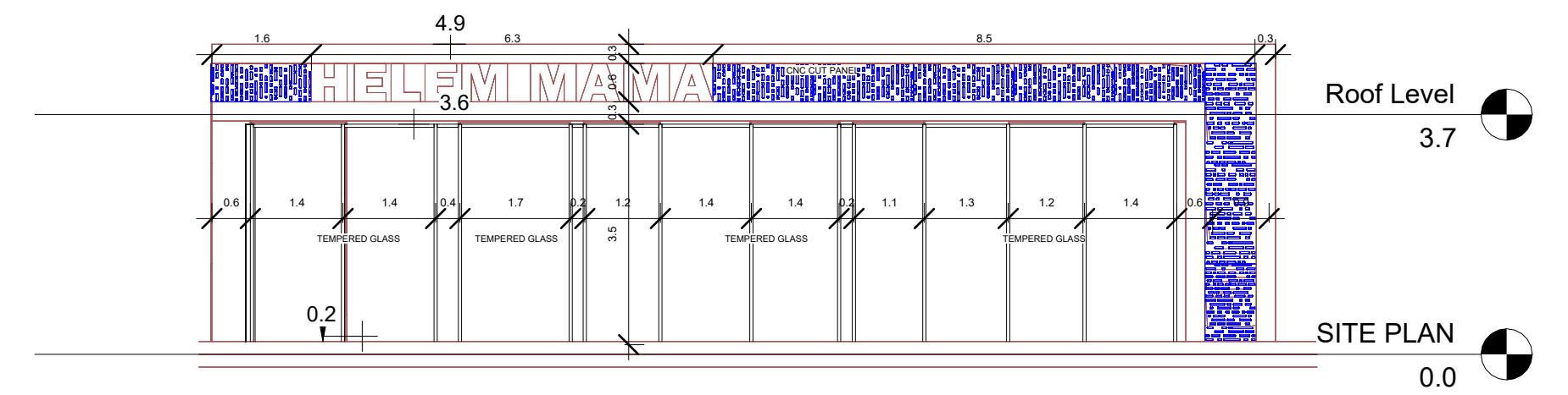
1 FRONT ELEVATION 1 : 100
