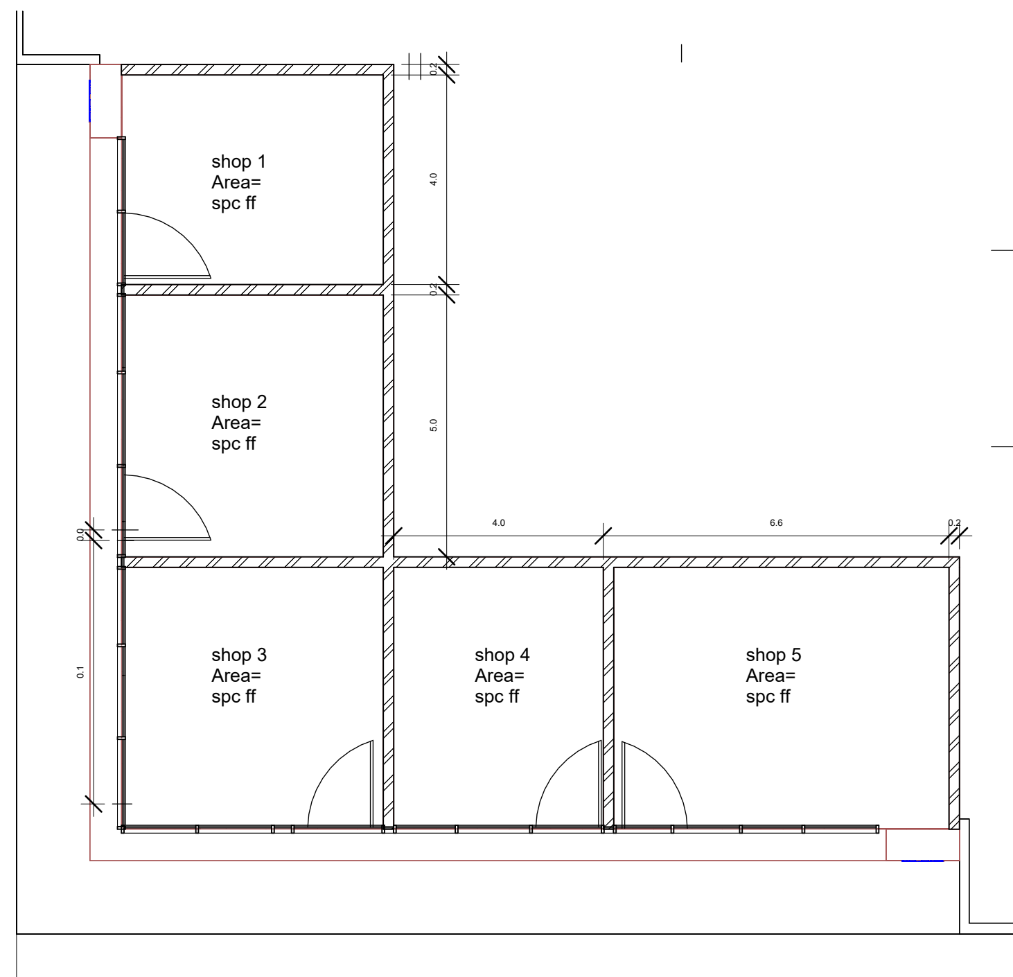
6 FLOOR PLAN 1:100
