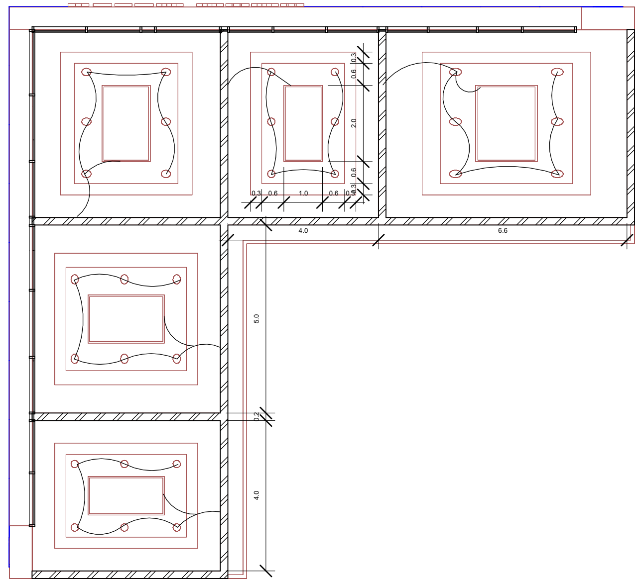
1 INSTALATION OF LIGHT AND SWITCH
